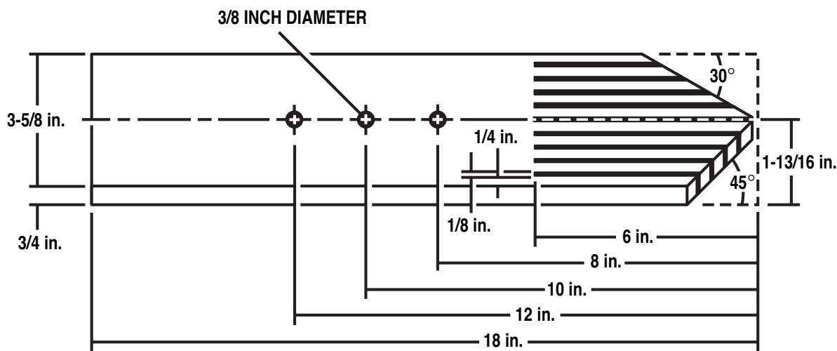
Figure 31: Featherboard
